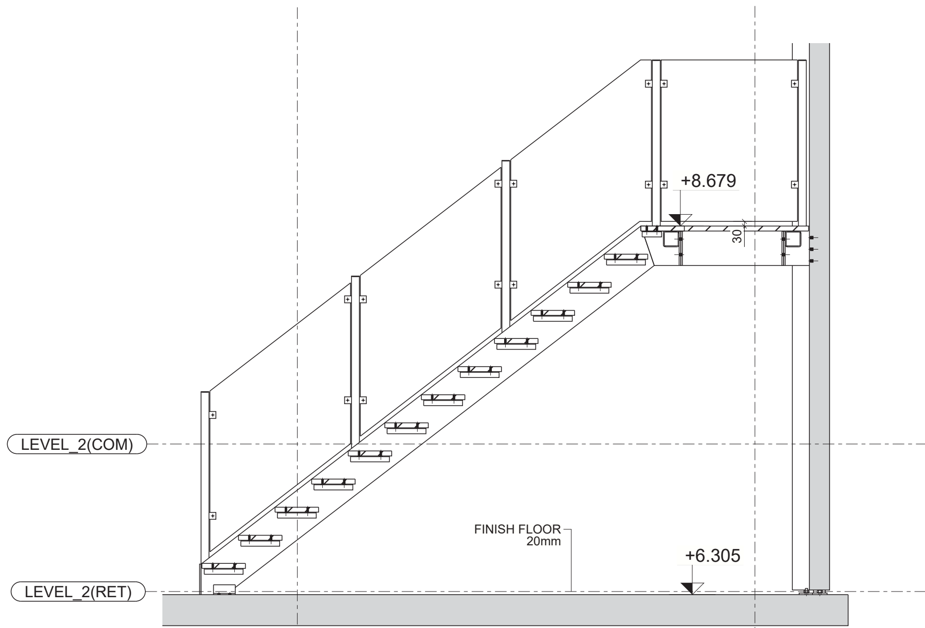
SECTION C-C E01
