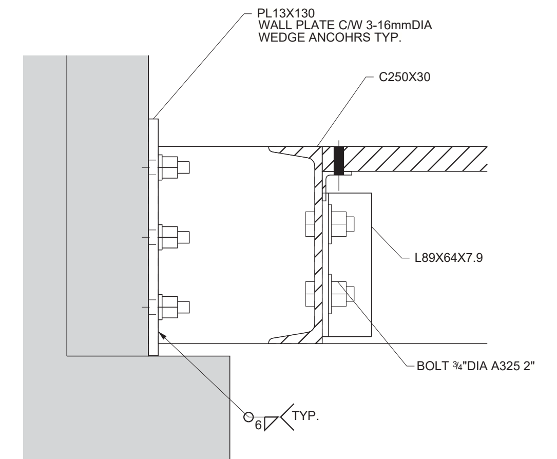
DETAIL D
