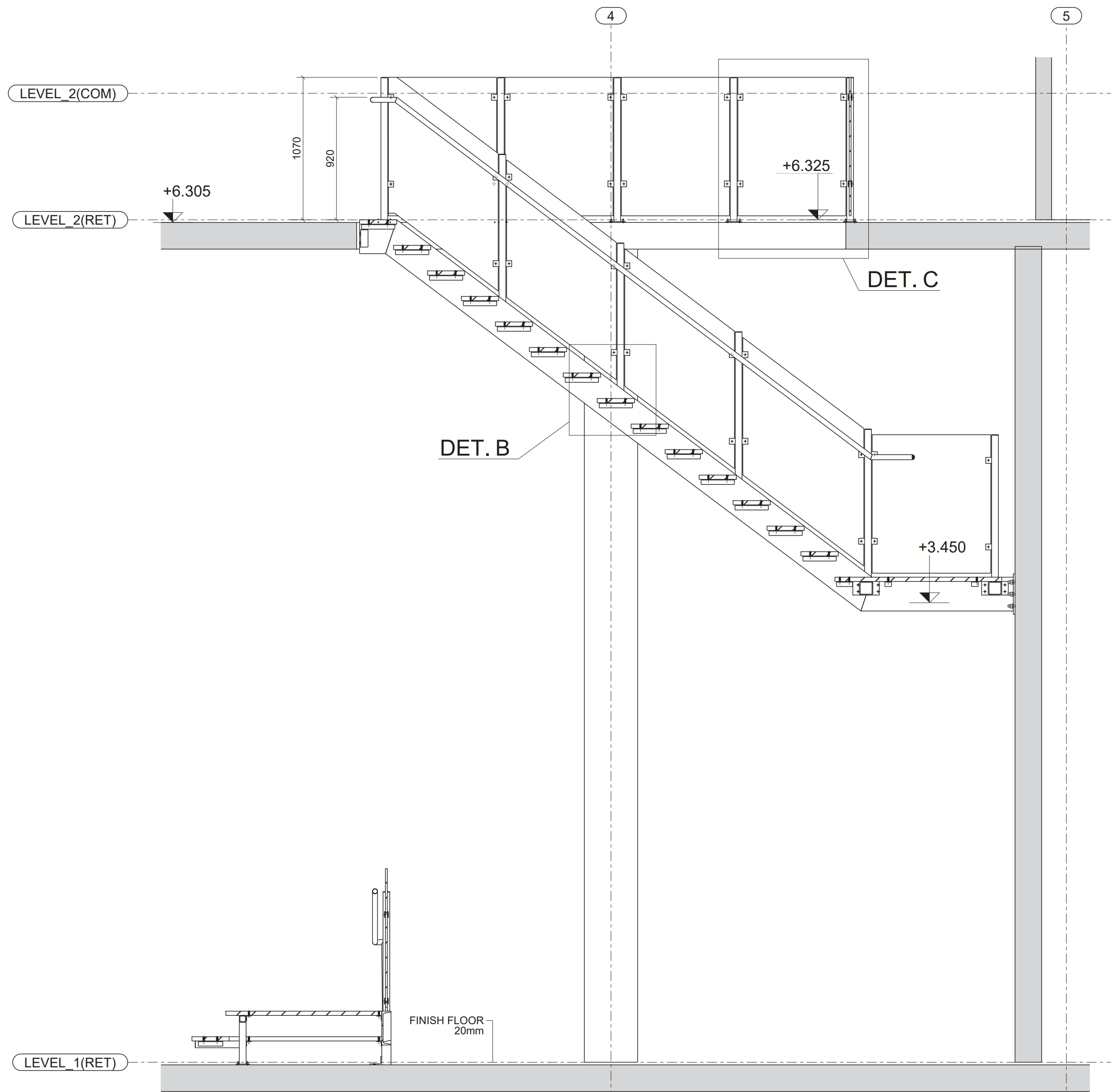
SECTION C-C E01
