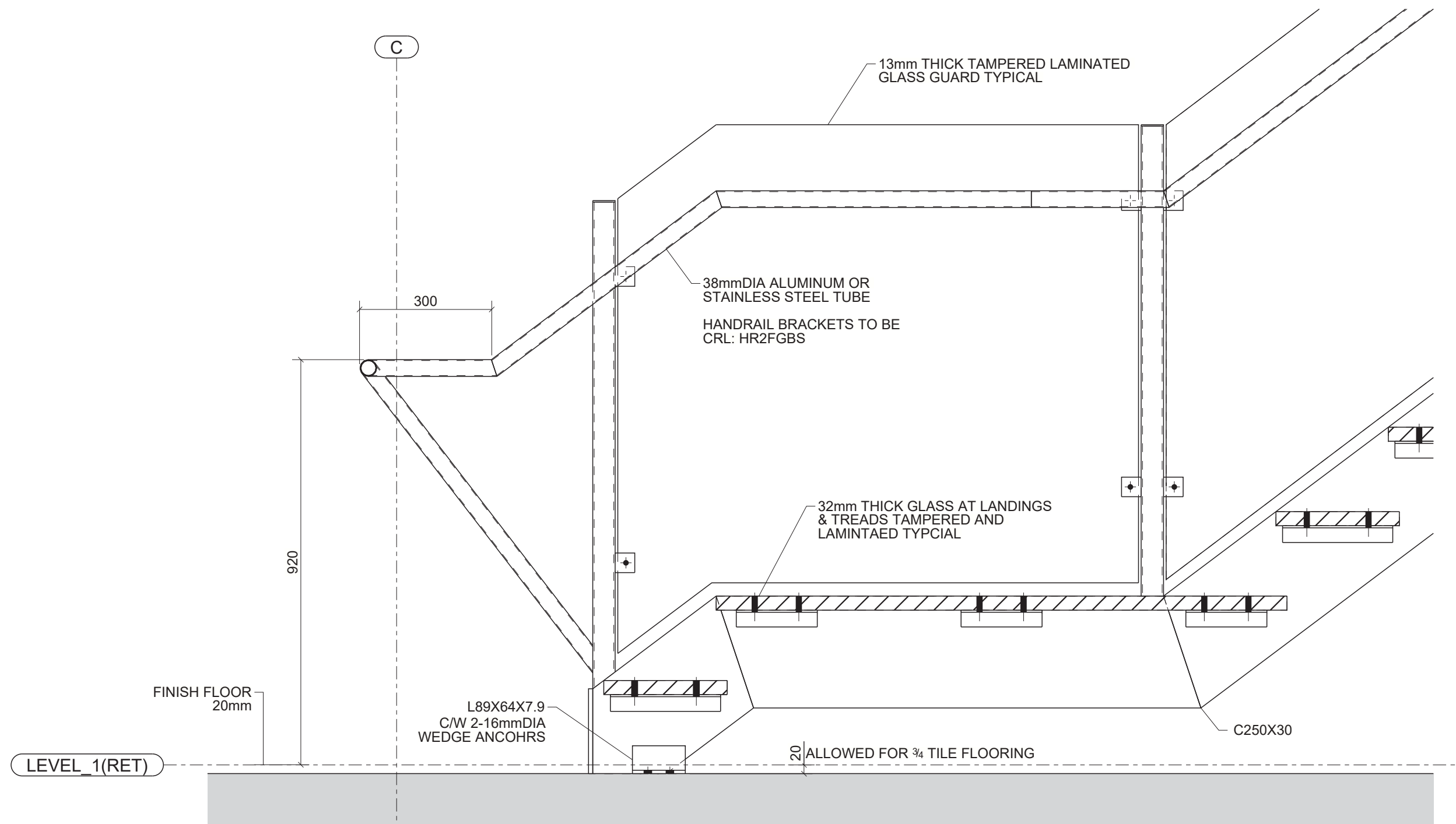
DETAIL A
