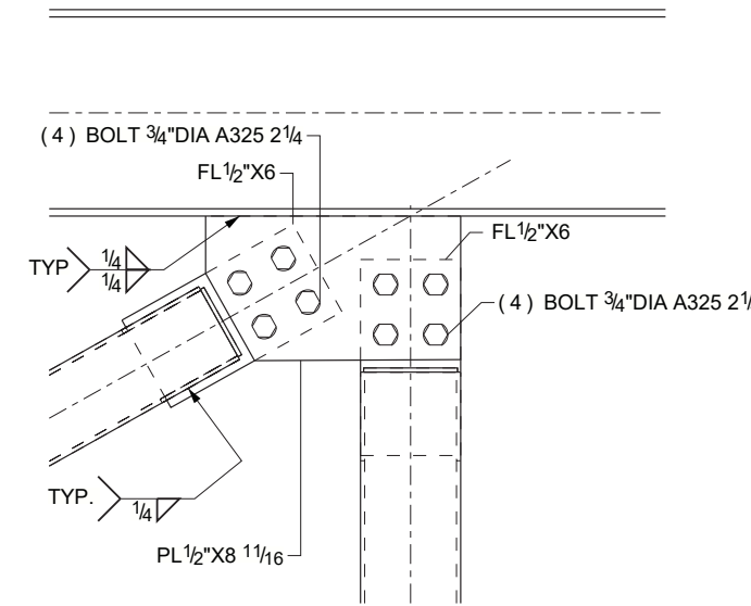
DETAIL F
