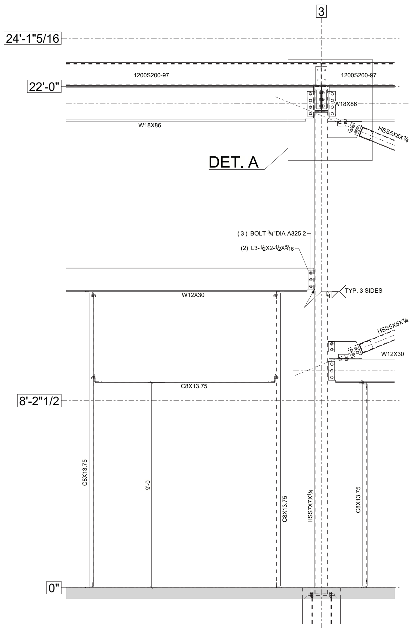
DETAIL A S-02
