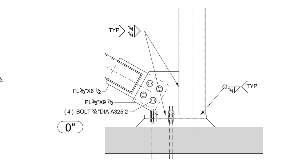
DETAIL G
