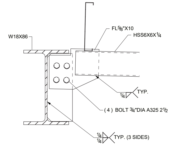
DETAIL I S-02
