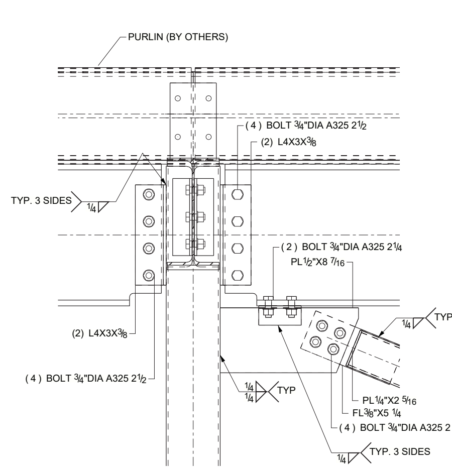
DETAIL E
