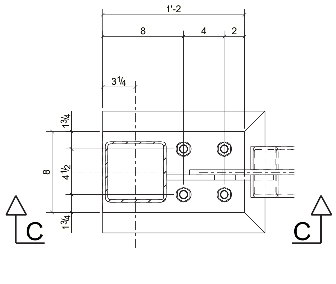
TYPICAL DETAIL [BPL-3]
