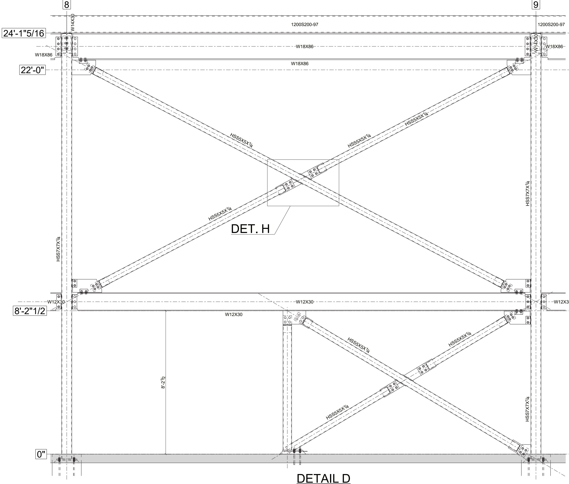
DETAIL D S-02
