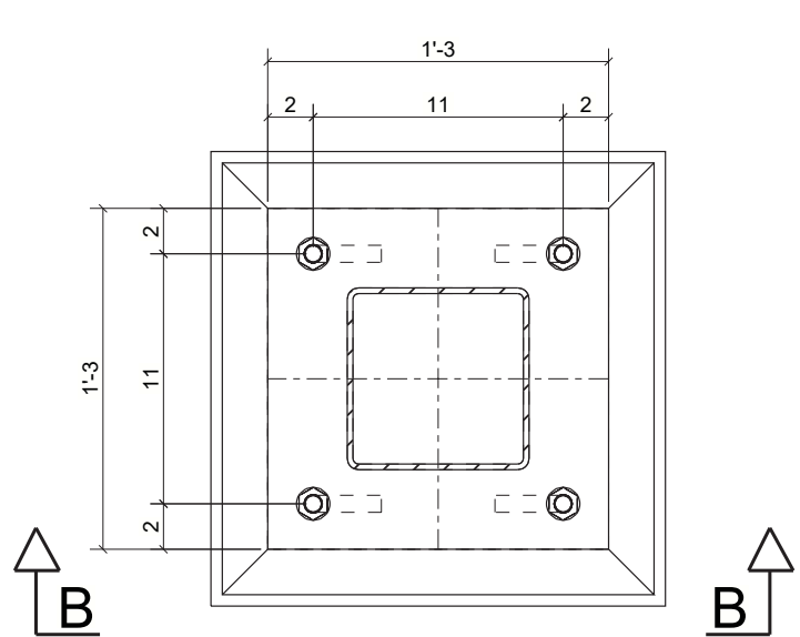
TYPICAL DETAIL [BPL-2]
