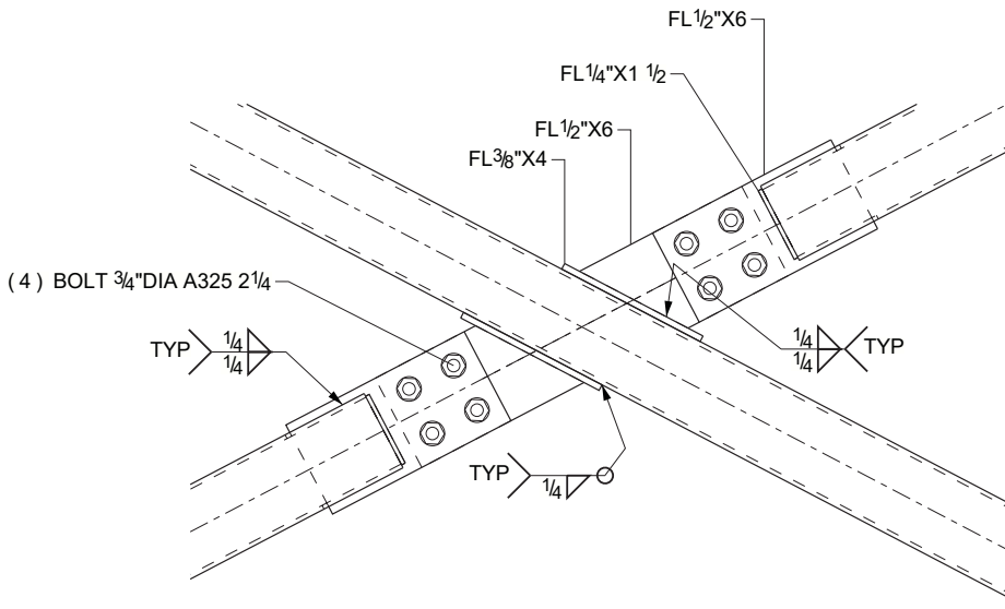
DETAIL H
