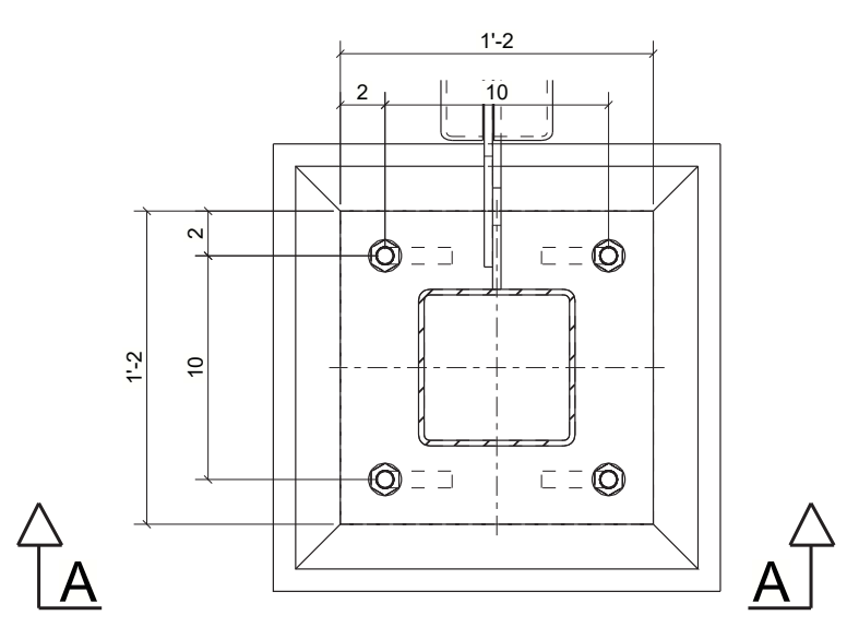
TYPICAL DETAIL [BPL-1]
