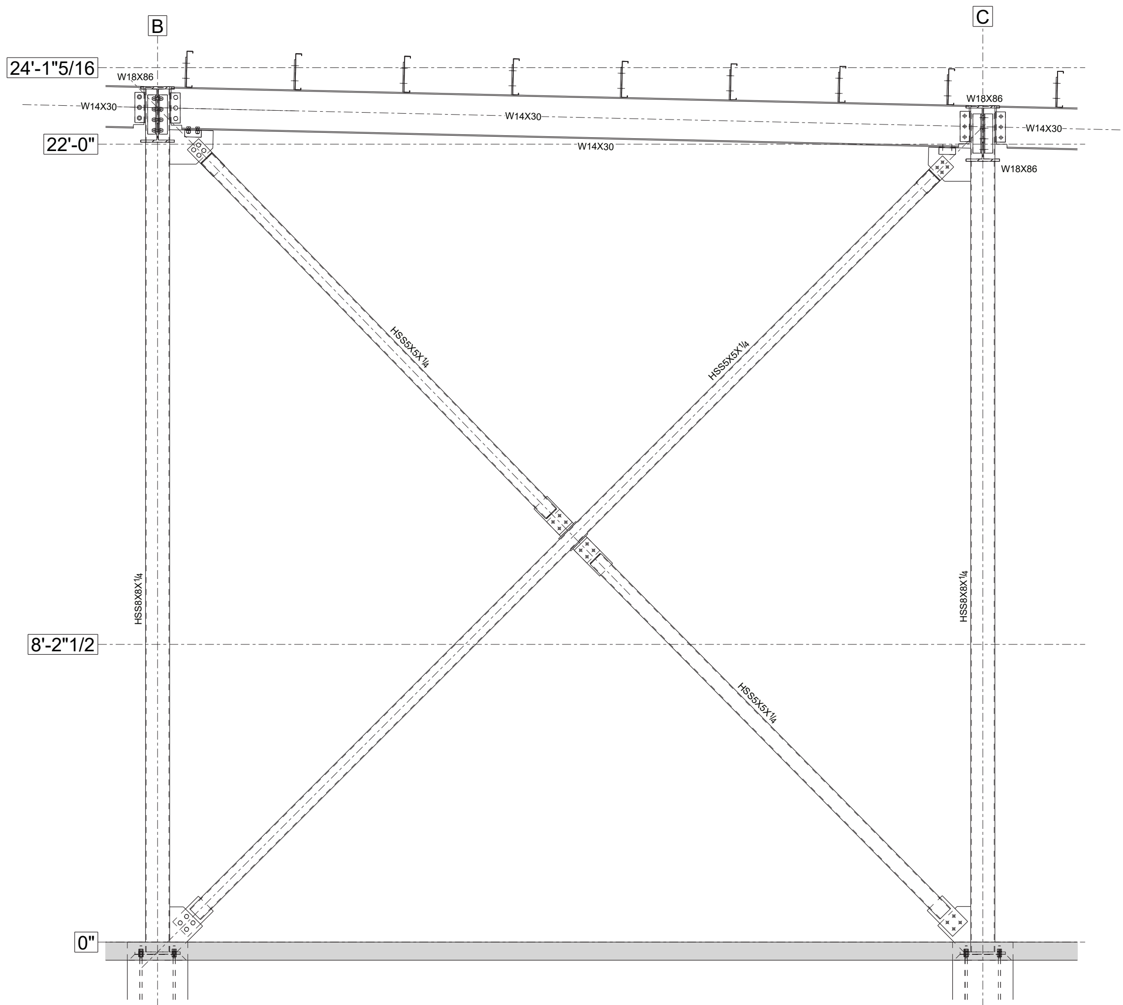
DETAIL C S-02
