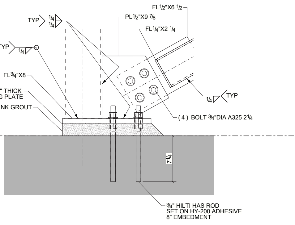
SECTION C-C
